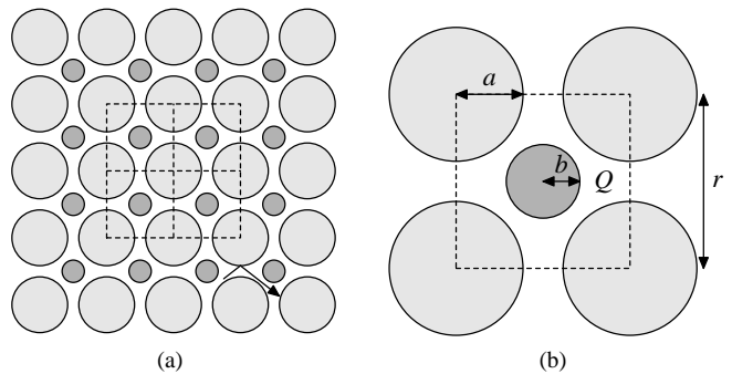
FIG. 1: (a) Part of the infinite system, constructed from two square lattices of disks shown in different shades of gray; dashed lines indicate several unit cells and an elastic collision is shown. (b) A single unit cell, defining the geometrical parameters. The billiard domain is the area Q exterior to the disks.
