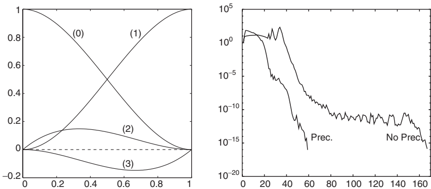
Fig. 8.17. Canonical Hermite basis on the reference interval 0 \leq \hat{x} \leq 1 ( left ); convergence histories for the conjugate gradient method in the solution of system (8.73) ( right ). On the x -axis the number of iterations k is shown, while the y -axis represents the quantity \|\mathbf{r}^{(k)}\|_2 / \|\mathbf{b}_1\|_2 , where \mathbf{r}^{(k)} is the residual of system (8.73) at the k -th iteration
