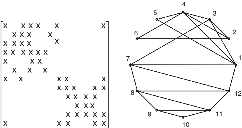
Fig. 3.3. Pattern of a symmetric sparse matrix (left) and of its associated graph (right). For the sake of clarity, the loops have not been drawn; moreover, since the matrix is symmetric, only one of the two sides associated with each a_{ij} \neq 0 has been reported
