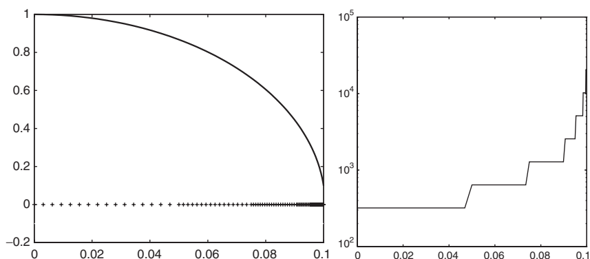
Fig. 9.7. Distribution of quadrature nodes ( left ); integration stepsize density in the approximation of integral (9.62) ( right )
