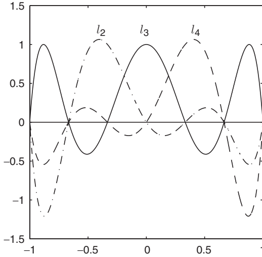
Fig. 8.1. Lagrange characteristic polynomials
