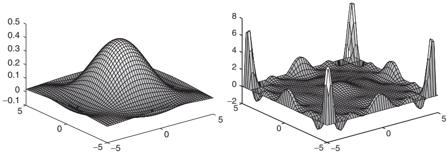
Fig. 8.5. Runge's counterexample extended to the two-dimensional case: interpolating polynomial on a 6 \times 6 nodes grid (left) and on a 11 \times 11 nodes grid (right). Notice the change in the vertical scale between the two plots
