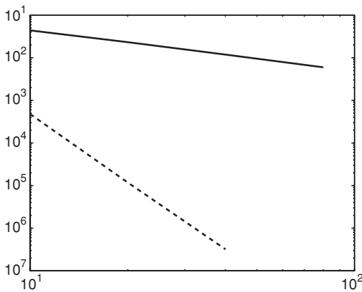
Fig. 13.1. Convergence analysis of the \theta -method as a function of the number 1/\Delta t of time steps (represented on the x -axis): \theta = 1 (solid line) and \theta = 0.5 (dashed line)
