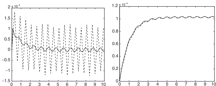
Fig. 11.14. Long-time behavior of the solution: velocities ( left ) and displacements ( right )
