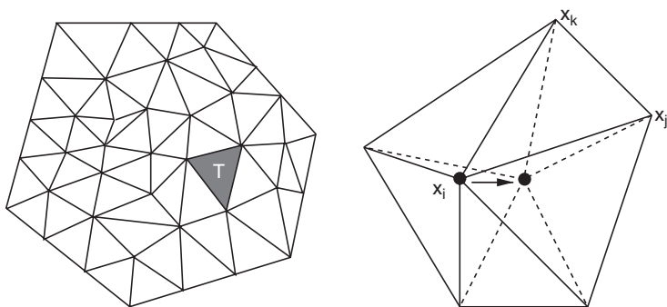
Fig. 3.13. An example of a decomposition into triangles of a polygonal domain D (left), and the effect of the barycentric regularization on a patch of triangles (right). The newly generated grid is plotted in dashed line
