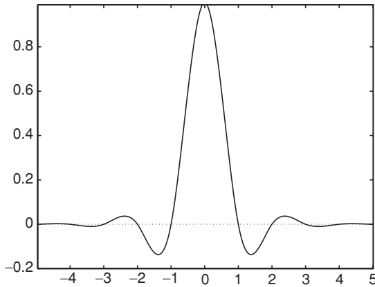
Fig. 8.9. Cardinal spline
