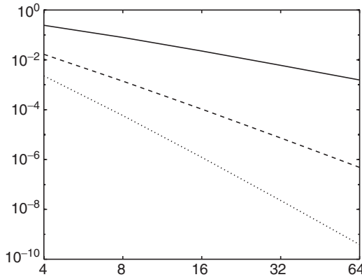
Fig. 10.5. Maximum nodal errors for the second-order centered finite difference scheme ( solid line ) and for the fourth ( dashed line ) and sixth-order ( dotted line ) compact difference schemes as functions of p = \log(n)
