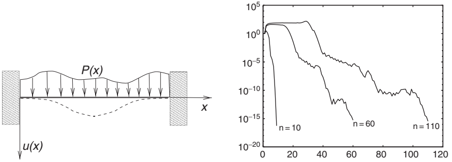
Fig. 4.15. Clamped beam (left); convergence histories for the preconditioned conjugate gradient method in the solution of system (4.78) (right)
