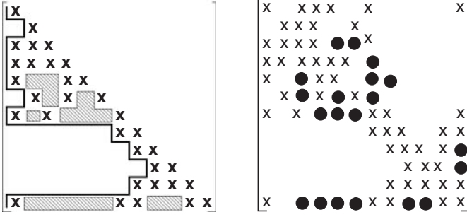
Fig. 3.4. The shaded regions in the left figure show the areas of the matrix that can be affected by fill-in, for the matrix considered in Figure 3.3. Solid lines denote the boundary of \mathcal{E}(A) . The right figure displays the factors that have been actually computed. Black dots denote the elements of A that were originally equal to zero
