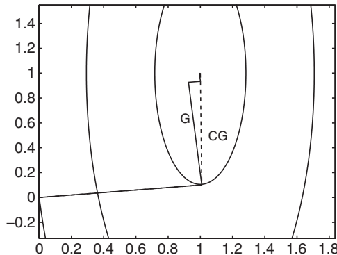
Fig. 4.7. Directions for the conjugate gradient method (denoted by CG, dashed line) and the gradient method (denoted by G, solid line). Notice that the CG method reaches the solution after two iterations
