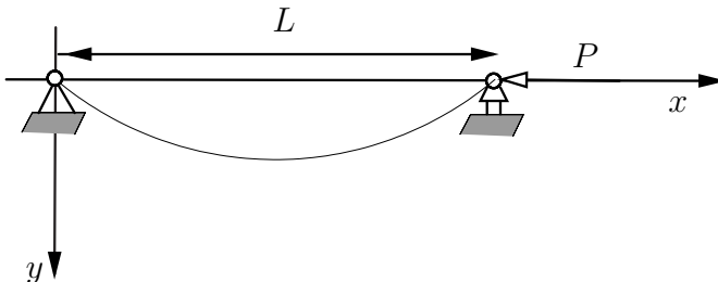
Fig. 5.4. A simply supported beam subject to a normal compression load
