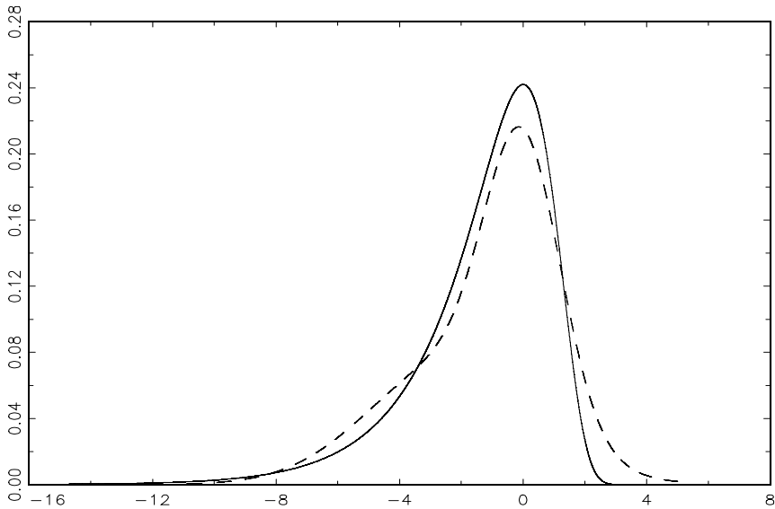
Figure 6.18 Density of the log of a \chi_1^2 as given by (6.189) (solid line) and the fitted normal mixture (dashed line) from the NYSE example.
