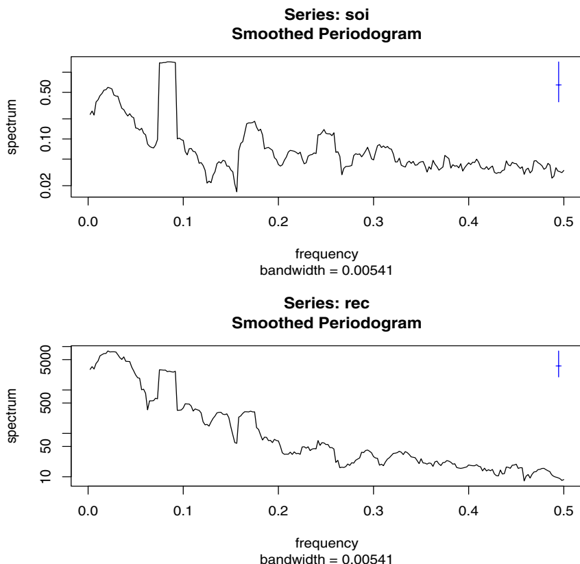
Figure 4.6 Figure 4.5 with the average periodogram ordinates plotted on a \log_{10} scale. The display in the upper right-hand corner represents a generic 95% confidence interval.
