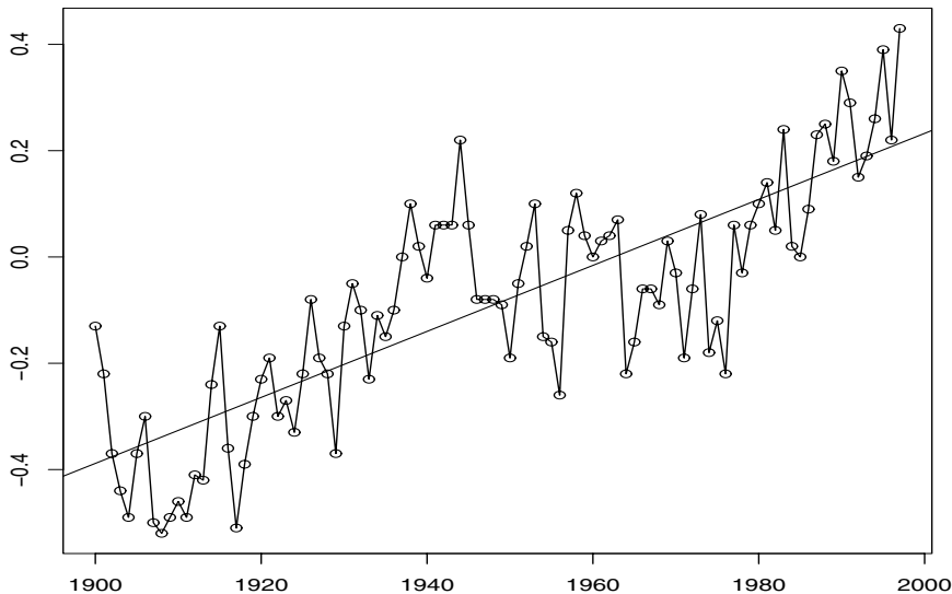
Figure 2.1 Global temperature deviations shown in Figure 1.2 with fitted linear trend line.
