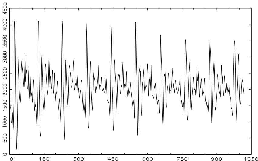
Figure 1.3 Speech recording of the syllable aaa...hhh sampled at 10,000 points per second with n = 1020 points.
