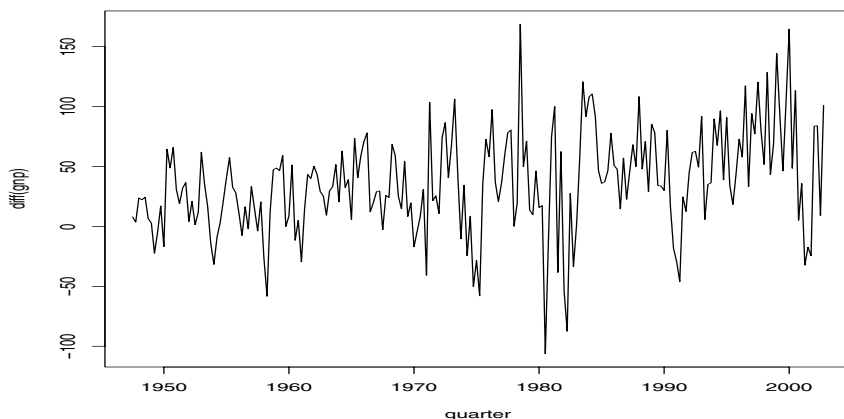
Figure 3.13 First difference of the U.S. GNP data.
