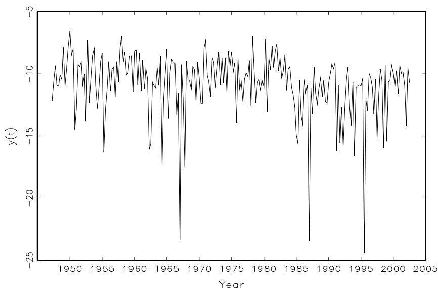
Figure 6.20 Log of the squared residuals from an MA(2) fit on GNP growth rate.
