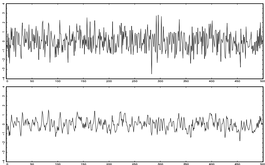
Figure 1.8 Gaussian white noise series (top) and three-point moving average of the Gaussian white noise series (bottom).
