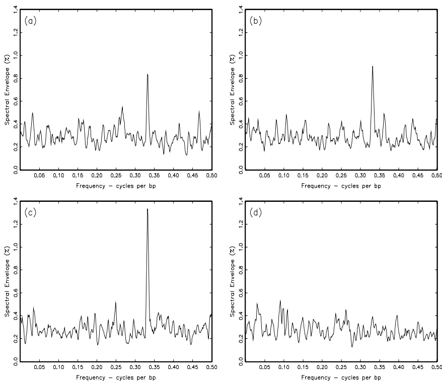
Figure 7.23 Smoothed sample spectral envelope of the BNR1 gene from the Epstein-Barr virus: (a) first 1000 bp, (b) second 1000 bp, (c) third 1000 bp, and (d) last 954 bp.
