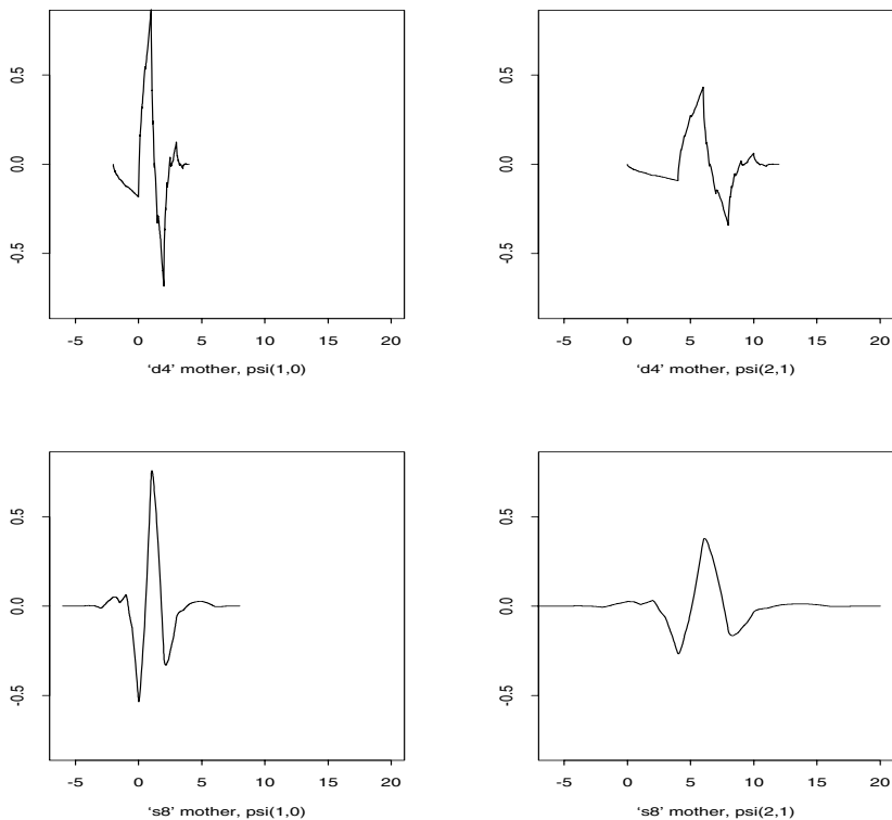
Figure 4.21 Scaled and translated daublet4 wavelets, \psi_{1,0}(t) and \psi_{2,1}(t) (top row); scaled and translated symmlet8 wavelets, \psi_{1,0}(t) and \psi_{2,1}(t) (bottom row).
