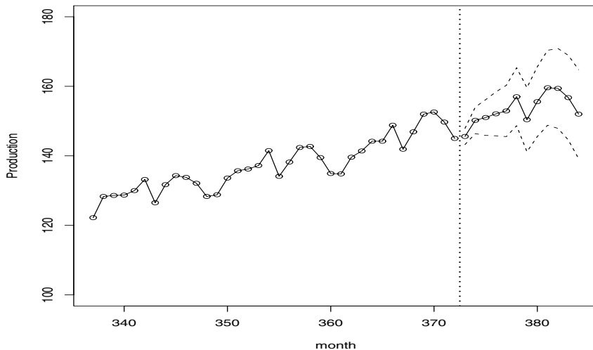
Figure 3.27 Forecasts and limits for production index. The vertical dotted line separates the data from the predictions.
