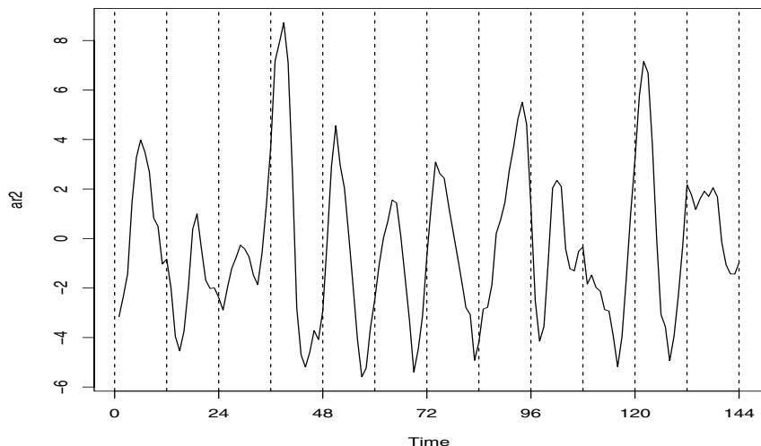
Figure 3.3 Simulated AR(2) model, n = 144 with \phi_1 = 1.5 and \phi_2 = -.75 .
