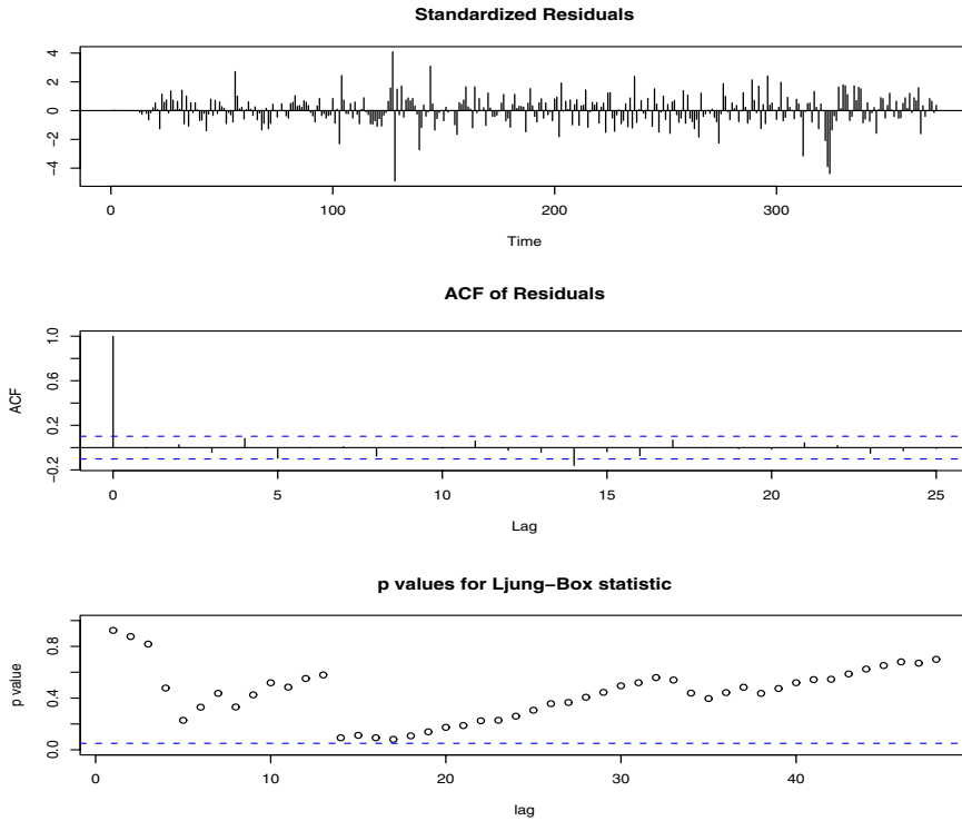
Figure 3.26 Diagnostics for the \text{ARIMA}(1, 1, 1) \times (2, 1, 1)_{12} fit on the Production data.
